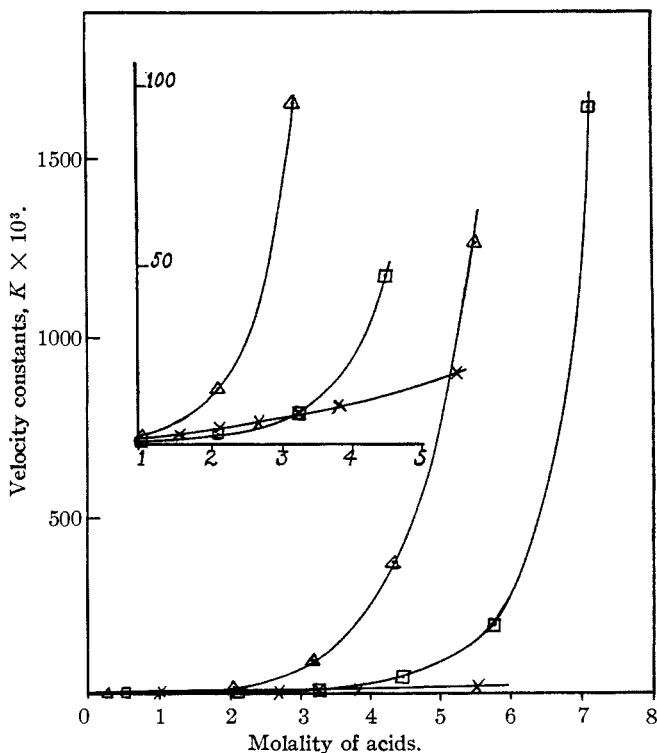
Fig. 1.—Plot of velocity constants K \times 10^3 against molality of acids: \Delta , HCl; \square HBr; \times , H 2 SO 4 .
